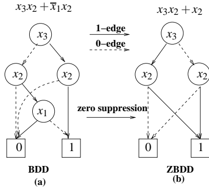
Figure 1: BDD versus ZBDD.
