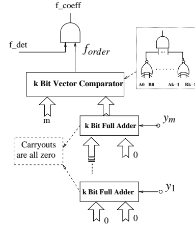
Figure 4: The logic circuit for coefficient generation in Theory 2
