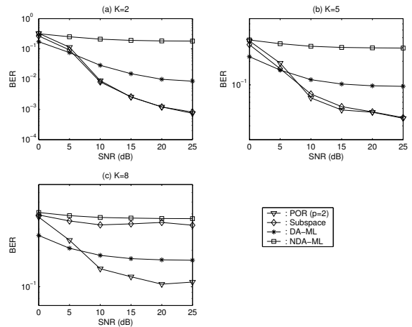
Fig. 4. BER comparison based on channel model CM2.
