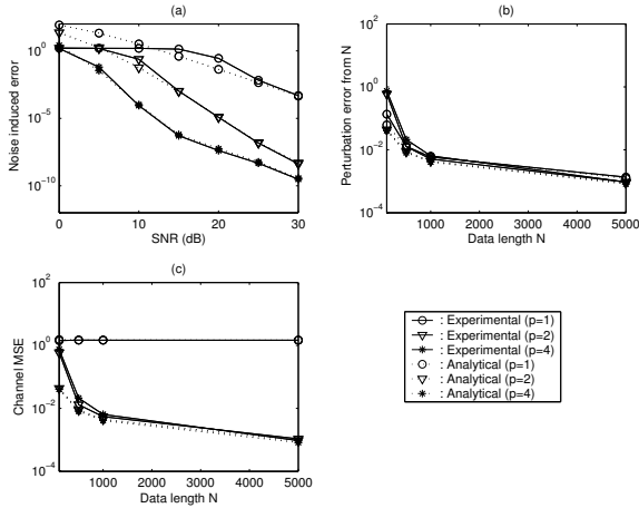
Fig. 1. Performance of channel estimation.
