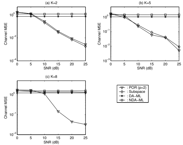
Fig. 3. Channel MSE comparison based on channel model CM2.
