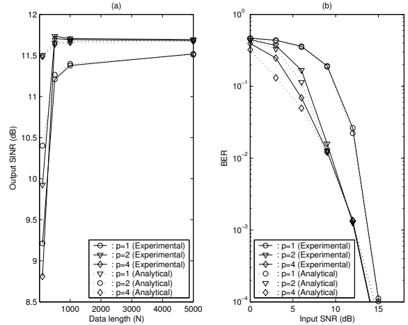
Fig. 2. Performance of symbol detection.
